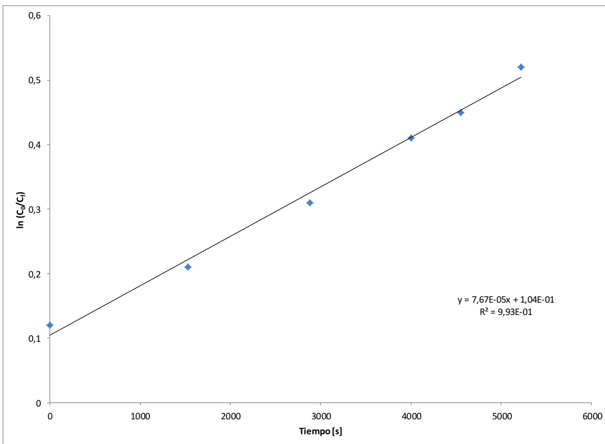
Figure 2S. Representation \ln C_0/C_t vs. different reaction times for thermal decomposition of ACDP in ethanol solution at 165 °C. Each point of the curve corresponds to the average of the determinations performed in triplicate
