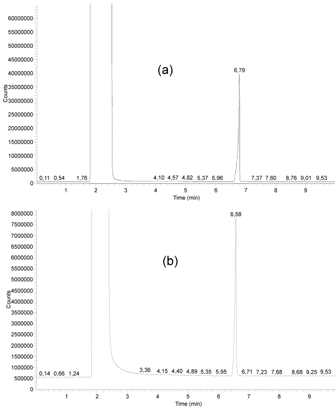
Figure 1S. Typical chromatograms for (a) DADP and (b) dDADP initial solutions
