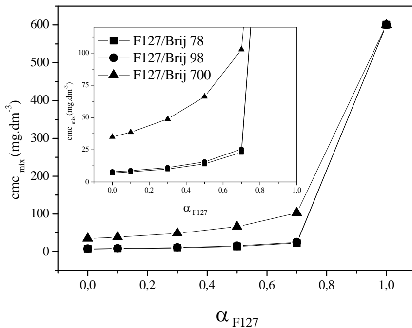
Figure 1S. Plots of mass fraction of F127 versus theoretical critical micelle concentration of F127/Brij 78, F127/Brij 98 and F127/Brij 700 mixtures at 37 °C
