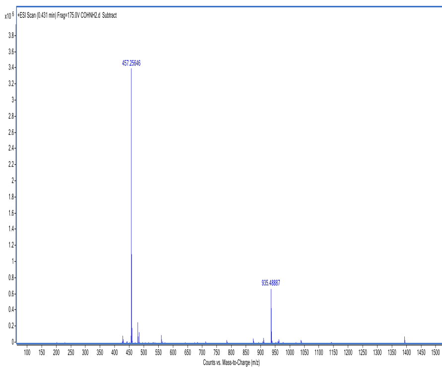
Figure 1S. MS of RBH
