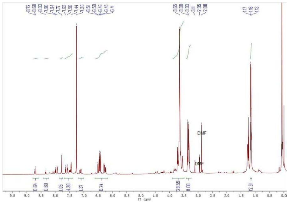
Figure 5S. ^1\text{H} NMR of P2
