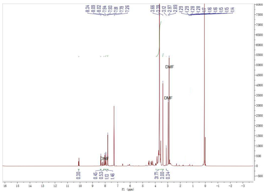
Figure 4S. ^1\text{H} NMR of P1
