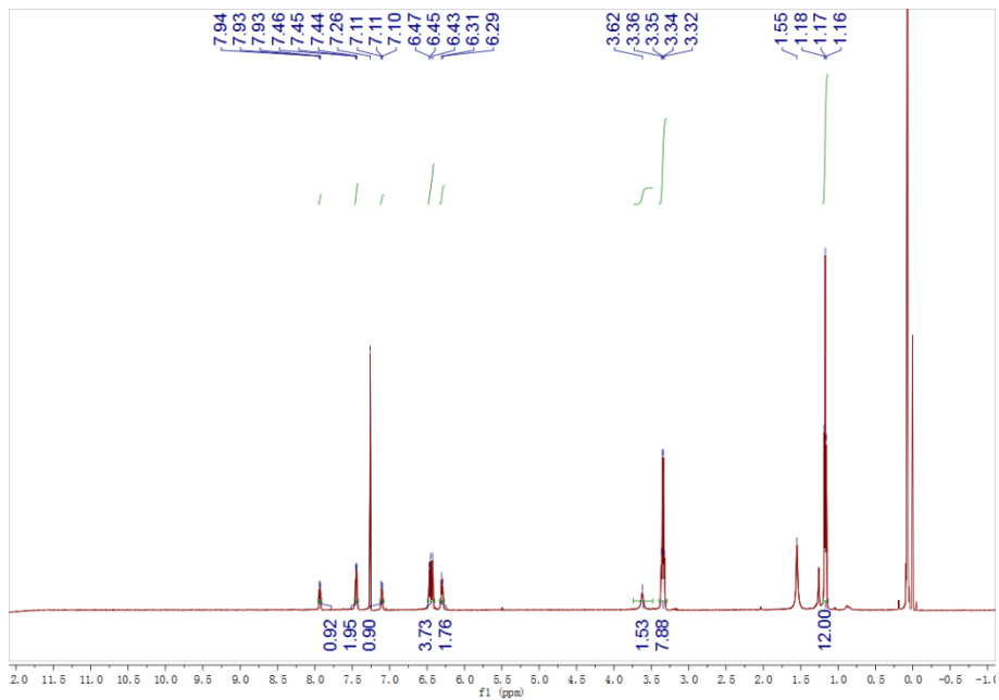
Figure 3S. ^1\text{H} NMR of RBH
