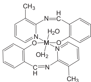
Figure 1. Proposed structure for all three complexes
