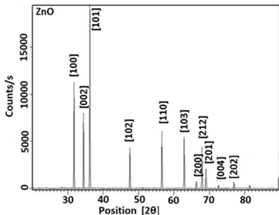
Figure 6. XRD spectra for ZnO nanoparticles
