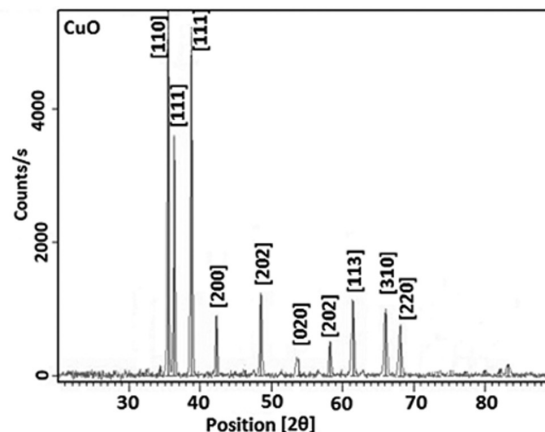
Figure 7. XRD spectra for CuO nanoparticles
