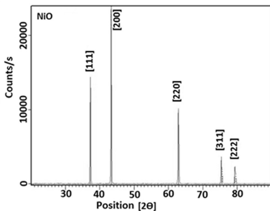
Figure 5. XRD spectra for NiO nanoparticles
