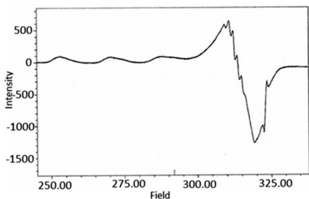
Figure 3. ESR spectra of complex ( C_1 ) in DMF at liquid nitrogen temperature
