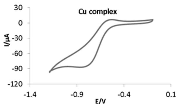
Figure 4. Cyclic voltammogram of copper(II) complex
