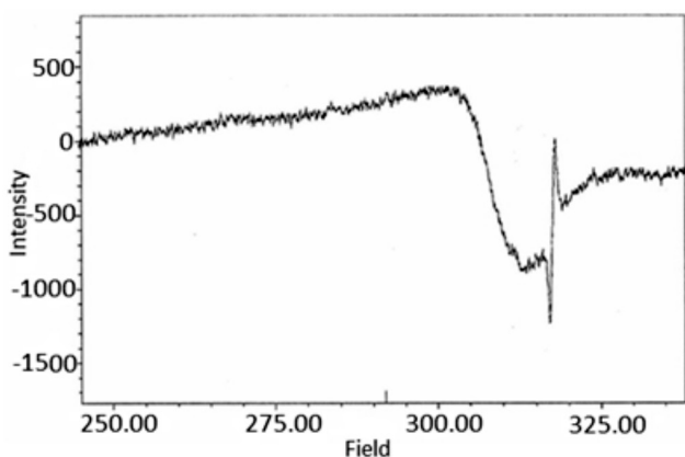
Figure 2. ESR spectra of complex ( C_1 ) in solid state at room temperature
