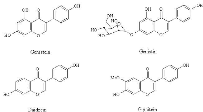
Figure 1. Chemical structures of isoflavones
