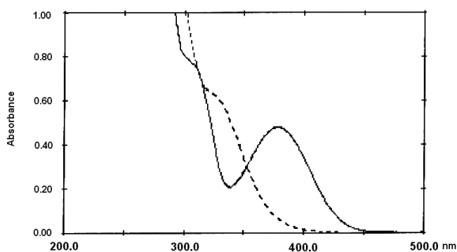
Figure 2. UV-Visible spectra of genistein in presence of \text{AlCl}_3 (full line) and absence of \text{AlCl}_3 (broken line) in methanol
